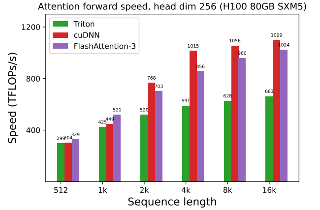
(b) Forward, with causal mask, head dim 256
